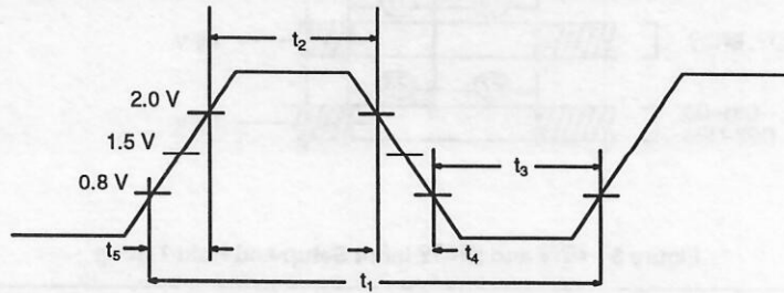
Figure 1 CLK Waveforms
