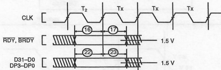
Figure 2 Input Setup and Hold Timing
