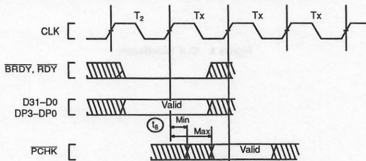
Figure 3 RDY and BRDY Input Setup and Hold Timing
