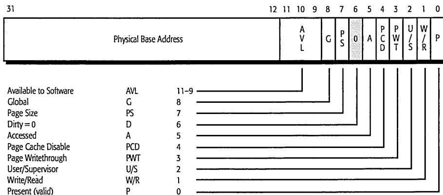
Figure 1-4. Page-Directory Entry (PDE)
