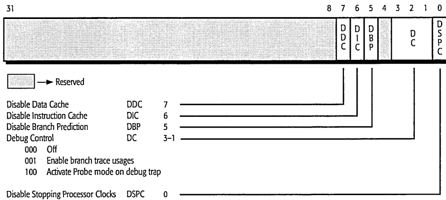
Figure 4-1. Hardware Configuration Register (HWCR)
