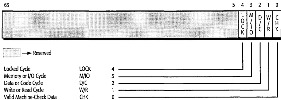
Figure 1-9. Machine-Check Type Register (MCTR)
