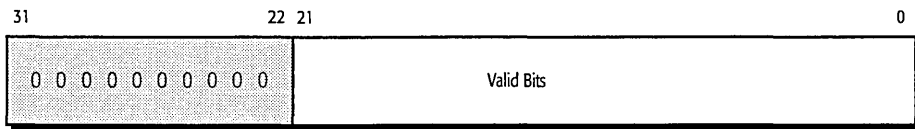
(E8h) 4-Kbyte Page and Status
