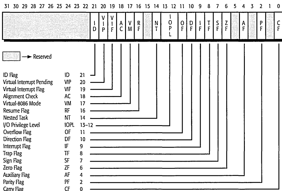
Figure 1-6. EFLAGS Register
