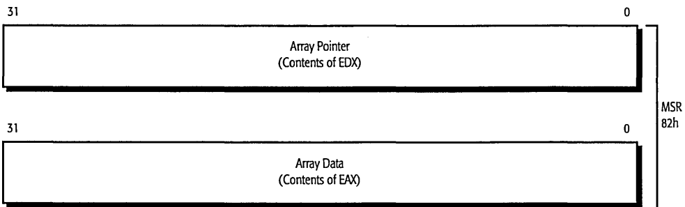
Figure 4-2. Array Access Register (AAR)
