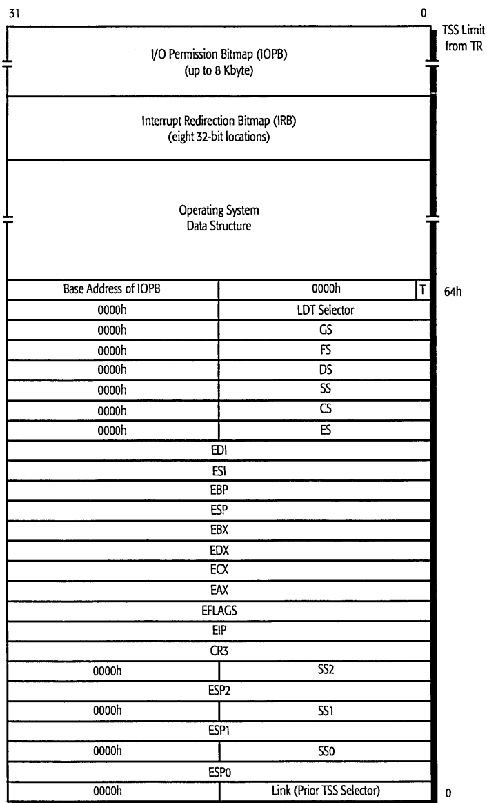
Figure 1-7. Task State Segment (TSS)
