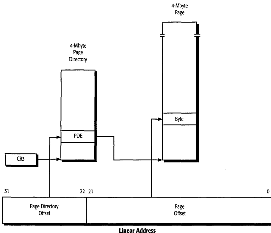
Figure 1-3. 4-Mbyte Paging Mechanism
