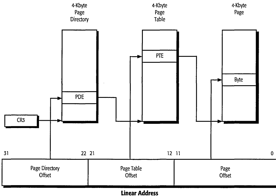
Figure 1-2. 4-Kbyte Paging Mechanism
