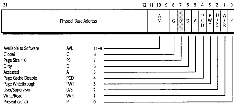
Figure 1-5. Page-Table Entry (PTE)
