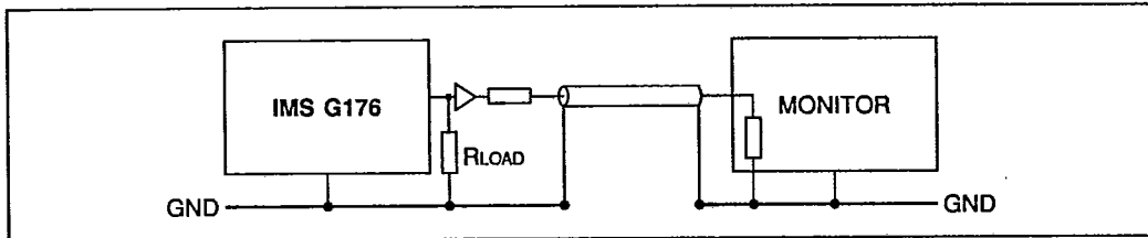
Figure 4.16 Buffered signal
