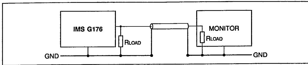
Figure 4.15 Double termination
