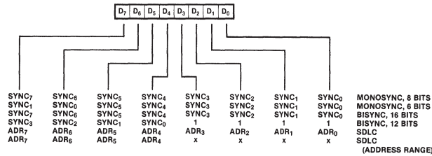
Figure 11. Write Register Bit Functions
