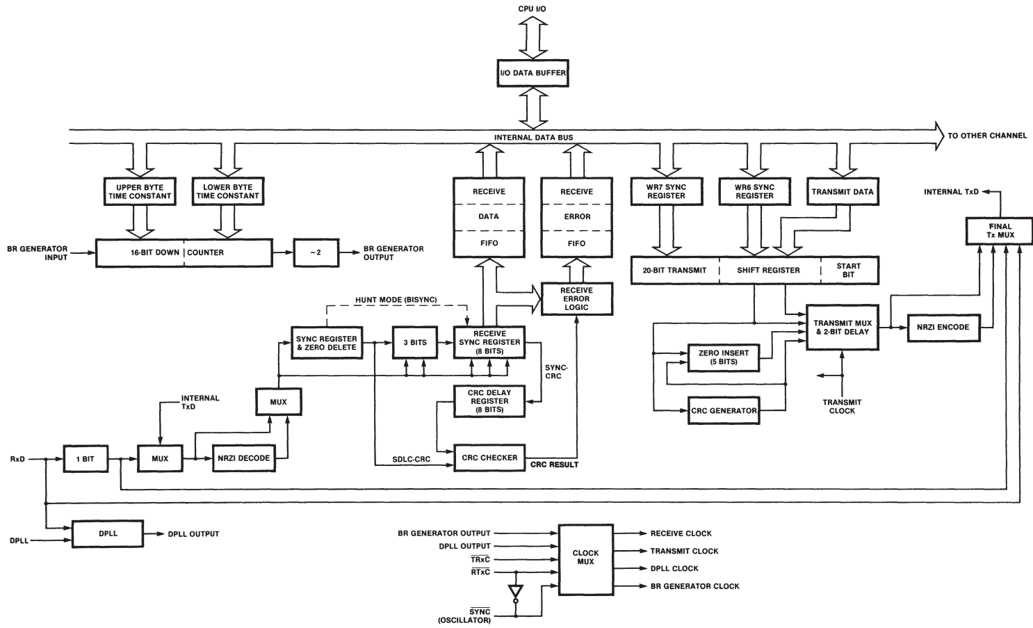
Figure 9. Data Path
